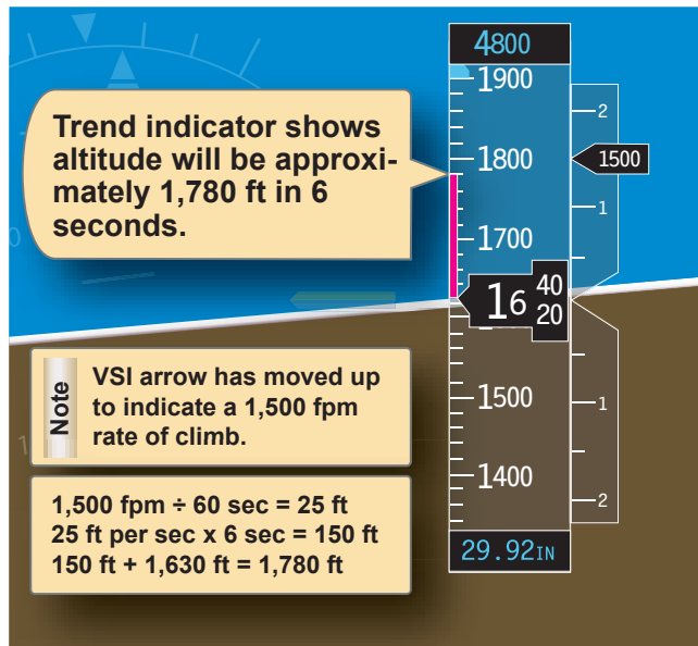
Figure 6-37. Altimeter trend indicators.
