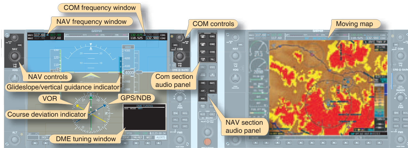
Figure 6-27. Navigation instruments.
