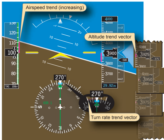
Figure 6-31. Supporting instruments.
