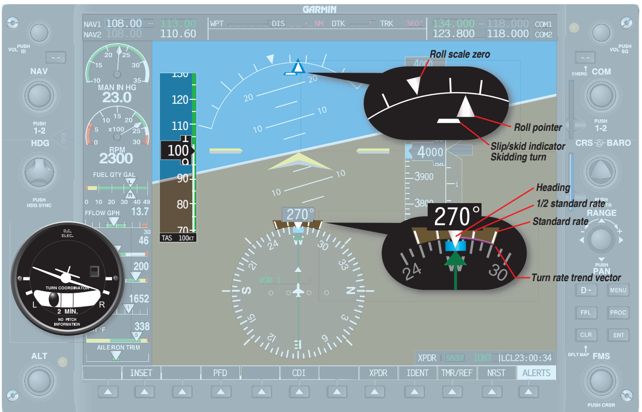
Figure 6-32. Primary bank.
