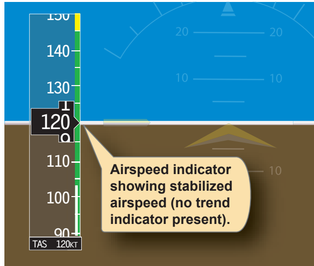
Figure 6-36. Airspeed indicators with no trend present.
